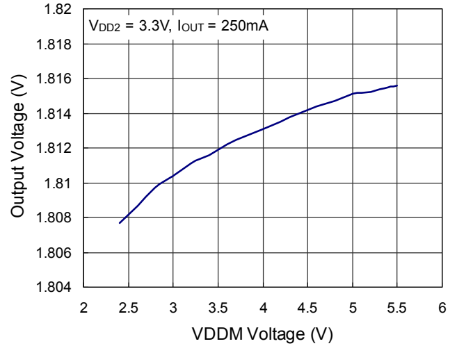
Buck2 Output Voltage vs. VDDM Voltage
