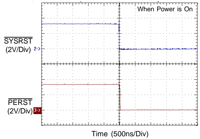
\overline{\text{PERST}} Asserted by \overline{\text{SYSRST}}
