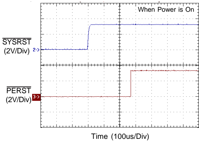
\overline{\text{PERST}} DE-Asserted by \overline{\text{SYSRST}}
